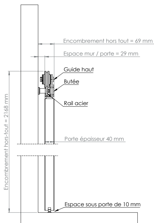
SCHEMA RAIL
